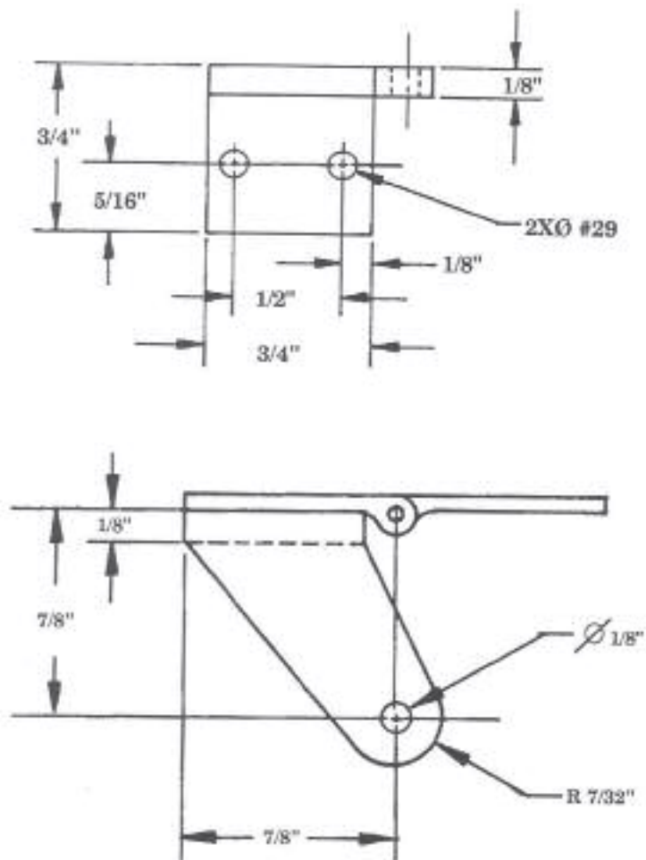
Trim tab hinge arm Figure 7b/G.6a
